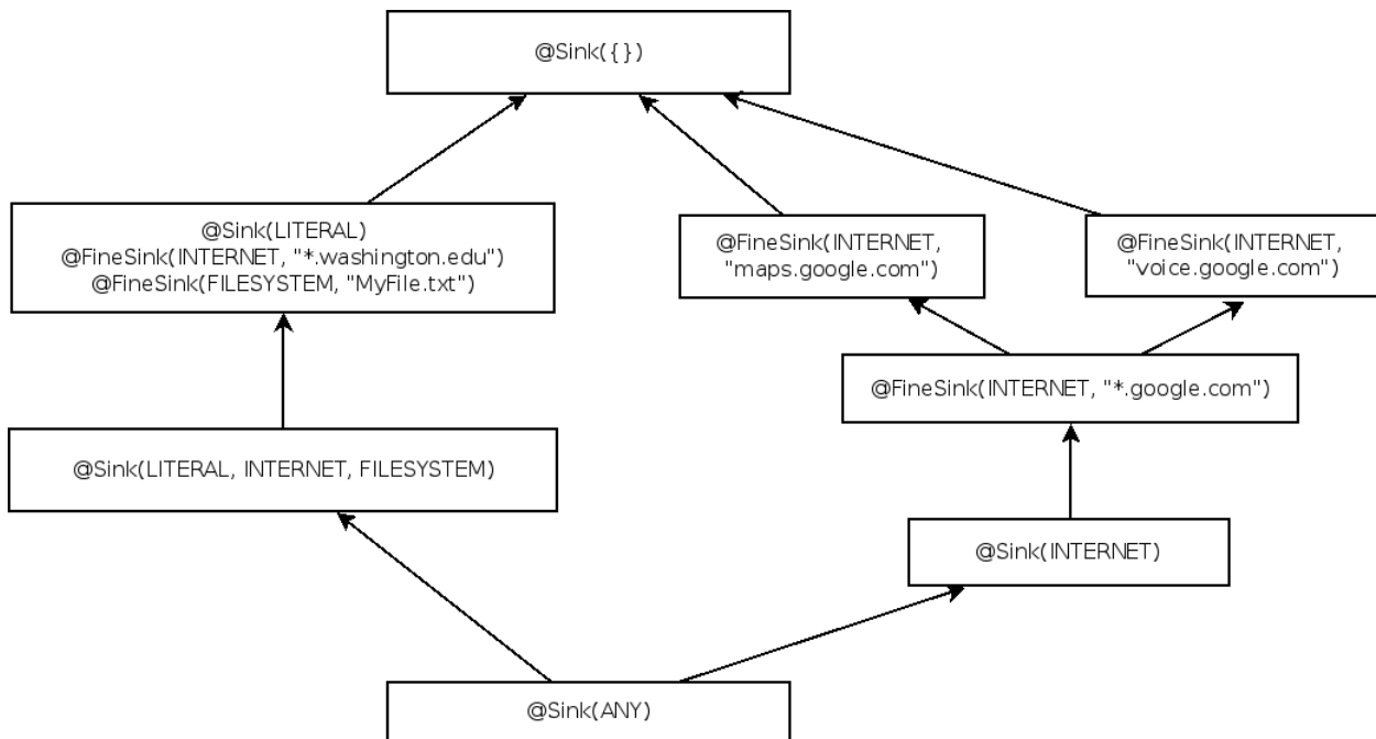
Figure 3.3: Partial qualifier hierarchy for parameterized flow sink type qualifiers, expressed as Java annotations @FineSink.
