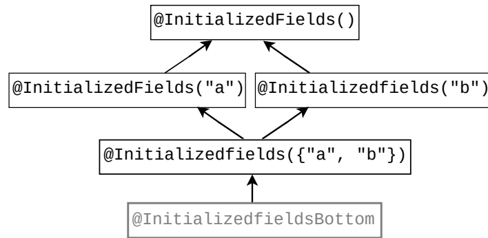
Figure 27.1: The type qualifier hierarchy of the Initialized Fields Checker. @InitializedFieldsBottom is rarely written by a programmer.
