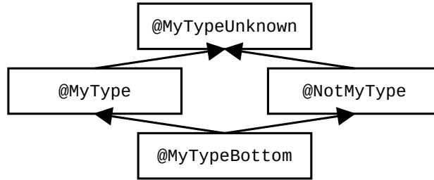
Figure 30.1: Type system for a type alias or typedef type system. The type system designer may choose to omit some of these types, but this is the general case. The type system designer’s choice of defaults affects the interpretation of unannotated code, which affects the guarantees given for unannotated code.
