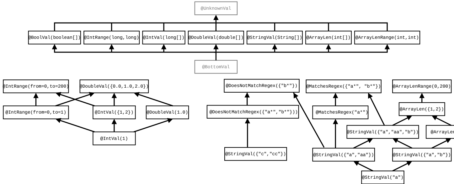
Figure 24.1: At the top, the type qualifier hierarchy of the Constant Value Checker annotations. The first four qualifiers are applicable to primitives and their wrappers; the next to Strings (it can also be written as @EnumVal for enumeration constants), and the final two to arrays. Qualifiers in gray are used internally by the type system but should never be written by a programmer. At the bottom are examples of additional subtyping relationships that depend on the annotations' arguments.
