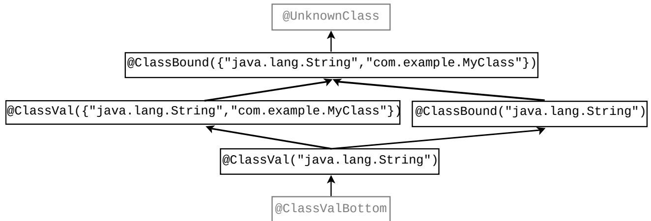
Figure 26.1: Partial type hierarchy for the ClassVal type system. The type qualifiers in gray (@UnknownClass and @ClassValBottom) should never be written in source code; they are used internally by the type system.
