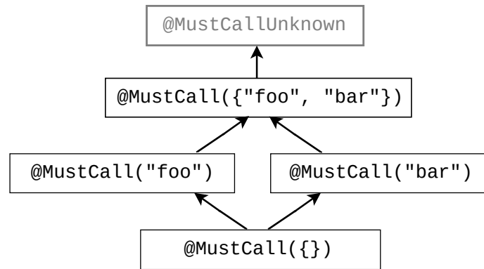
Figure 29.1: Part of the Must Call Checker’s type qualifier hierarchy. The full hierarchy contains one @MustCall annotation for every combination of methods. Qualifiers in gray are used internally by the type system but should never be written by a programmer.
