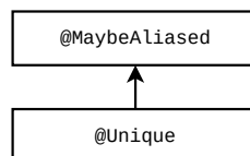
Figure 28.1: Type hierarchy for the Aliasing type system. These qualifiers are applicable to any reference (non-primitive) type.
