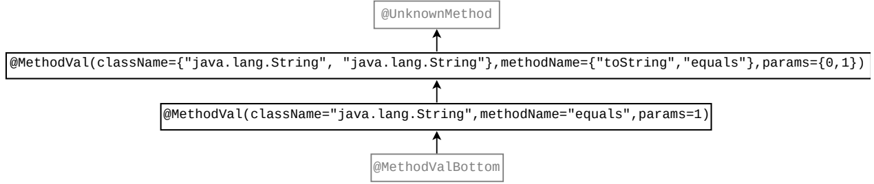
Figure 26.2: Partial type hierarchy for the MethodVal type system. The type qualifiers in gray (@UnknownMethod and @MethodValBottom) should never be written in source code; they are used internally by the type system.
