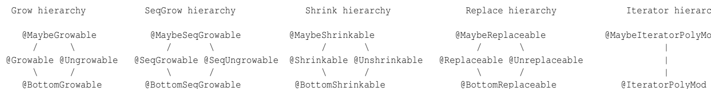
Figure 22.1: Independent modifiability qualifier hierarchies. Each annotated type carries one qualifier from each hierarchy.
