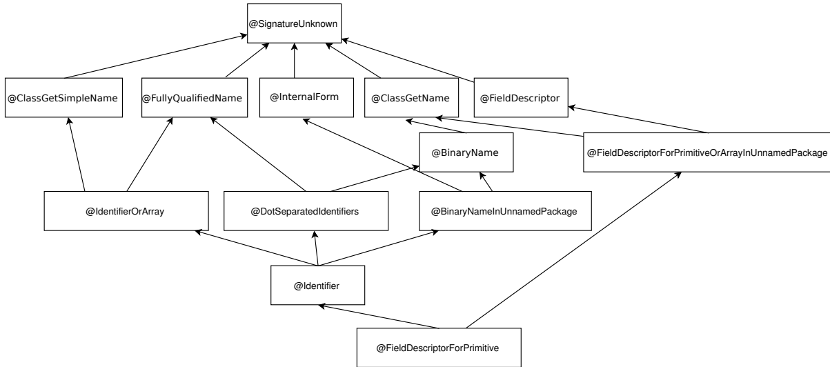
Figure 15.1: Partial type hierarchy for the Signature type system, showing string representations of a Java type. The type qualifiers are applicable to CharSequence and its subtypes. Programmers only need to write the boldfaced qualifiers, in the second row; qualifiers below those are included to improve the internal handling of String literals.
