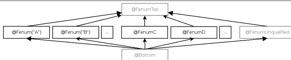
Figure 8.1: Partial type hierarchy for the Fenum type system. There are two forms of fake enumeration annotations — above, illustrated by @Fenum("A") and @FenumC . See section 8.1 for descriptions of how to introduce both types of fenums. The type qualifiers in gray ( @FenumTop , @FenumUnqualified , and @Bottom ) should never be written in source code; they are used internally by the type system.
