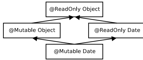
Figure 4: Type hierarchy for Javari's ReadOnly type qualifier.
